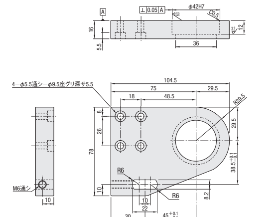
PLHDB-RE-FJ-L
