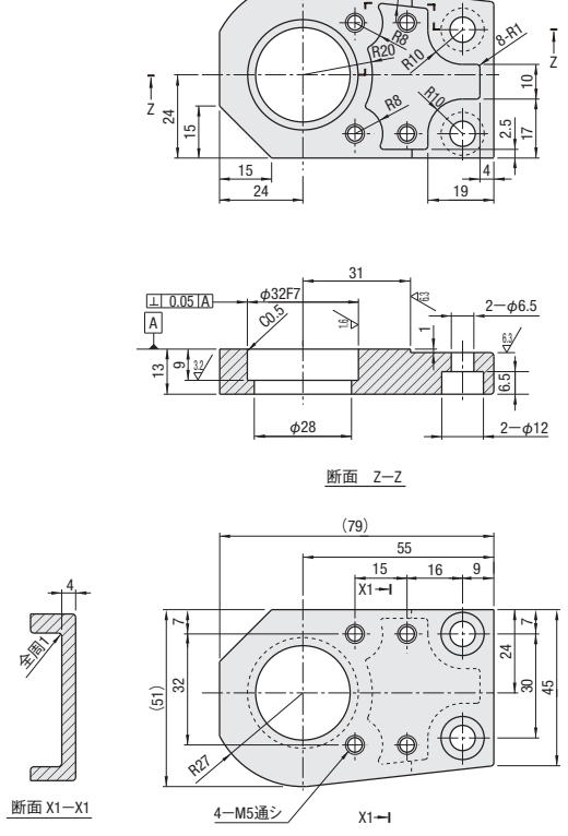
PLHDB-RE-TDK-L
