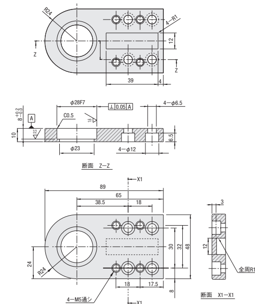
PLHDB-RE-FG-R
