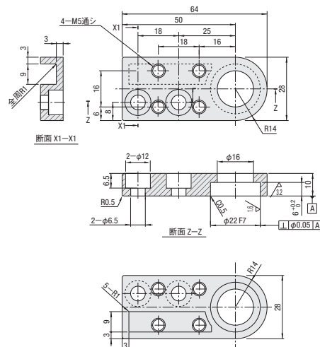
PLHDB-RE-FG-L
