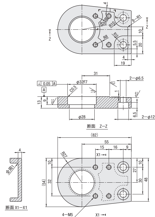
PLHDB-RE-TD-R
