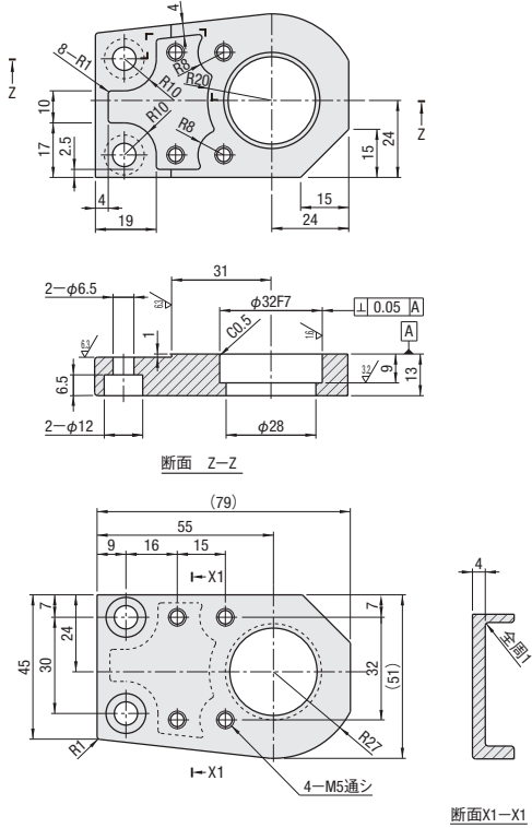
PLHDB-RE-TD-L
