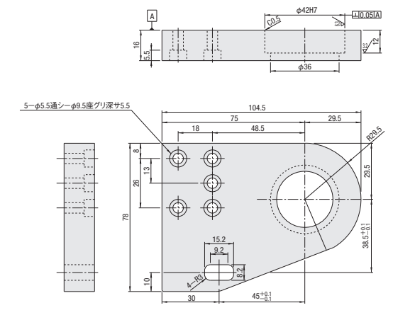
PLHDB-RE-FJ-L
