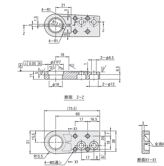
PLHDB-RE-TC-R
