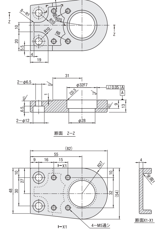
PLHDB-RE-TDK-R
