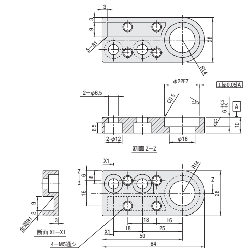
PLHDB-RE-FG-R
