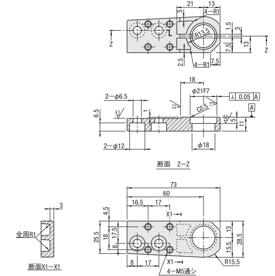
PLHDB-RE-TC-L
