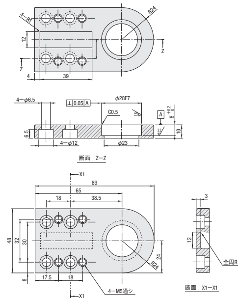
PLHDB-RE-FG-L
