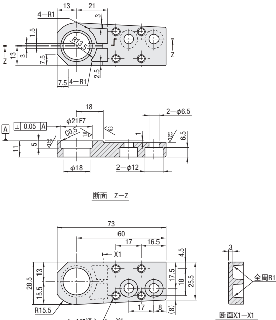
PLHDB-RE-TCK-L
