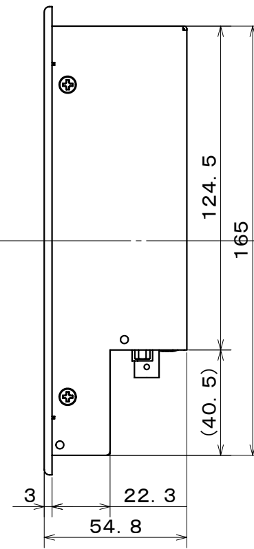
Right-side View
