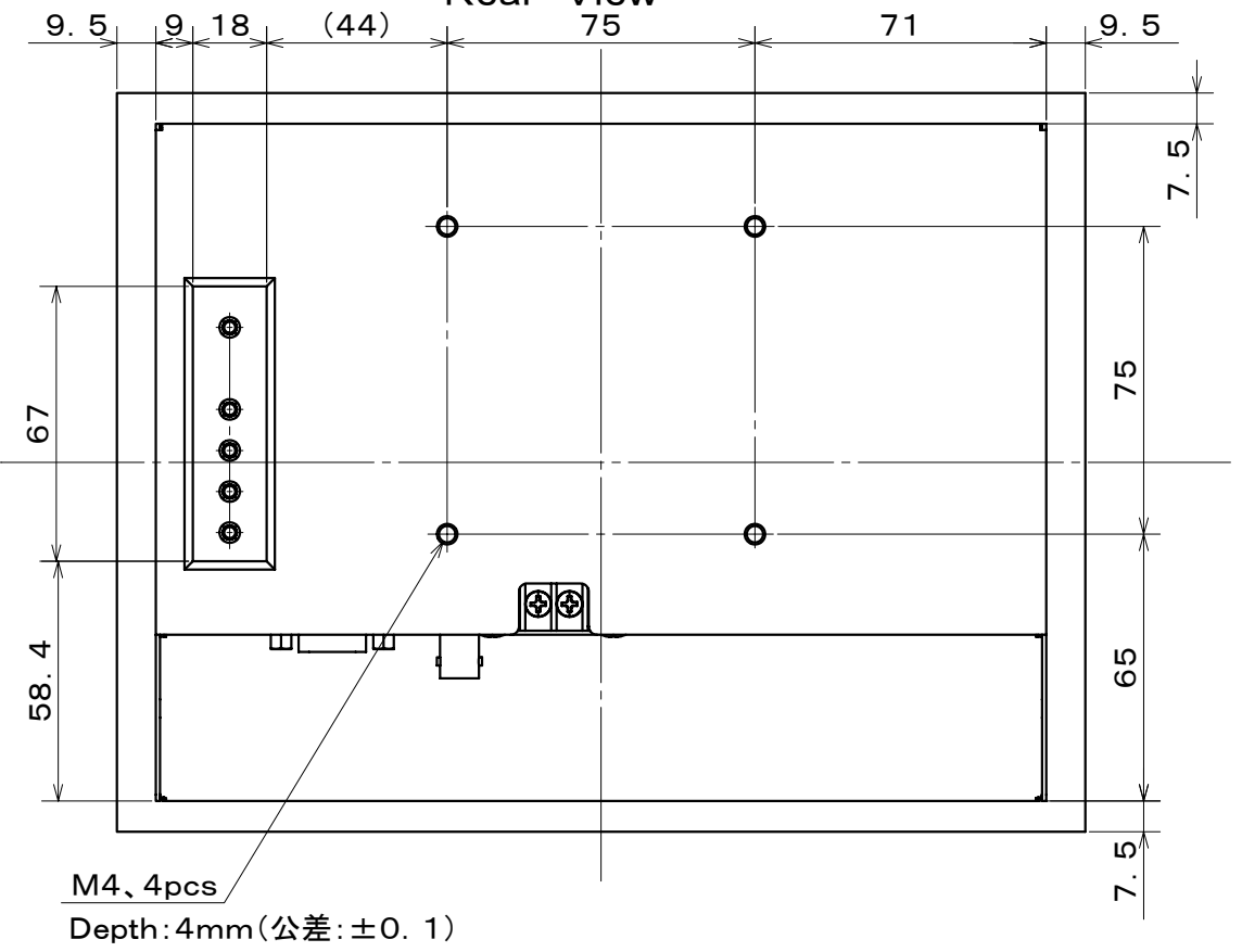
Rear View
