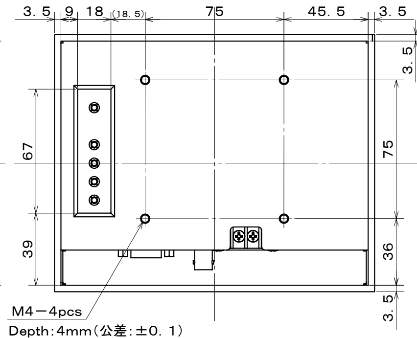
Rear View
