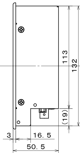
Right-side View
