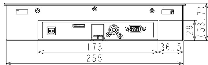
Bottom View
