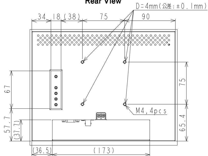
Rear View
