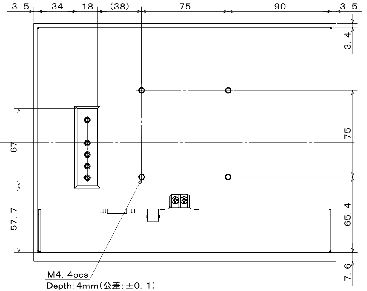
Rear View
