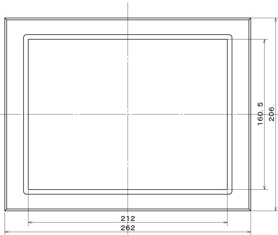
Front View
