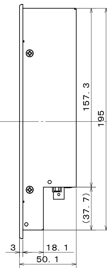
Right-side View
