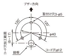
MST-LME-02*** (Φ60)
