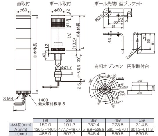
MST-LME-02*** (Φ60)
